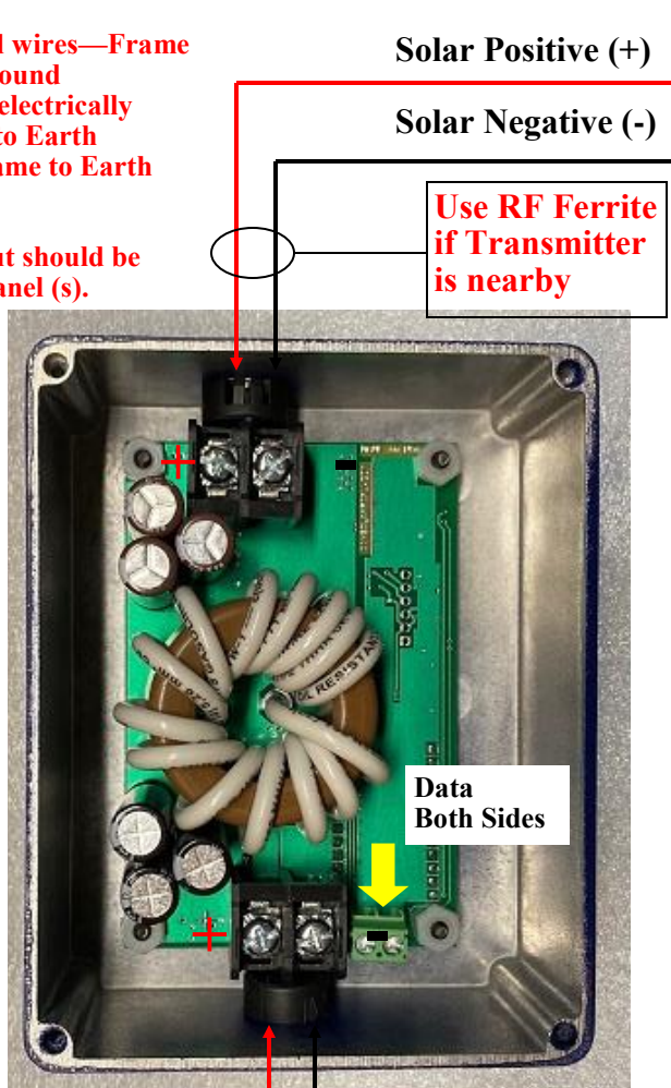
36 to 80 Cell Solar Panel
